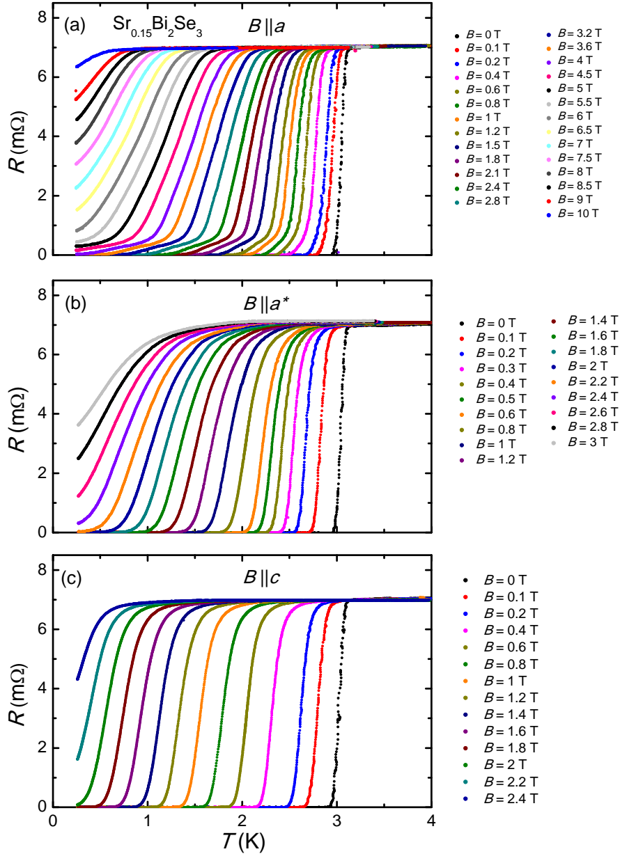
Fig. S6 Superconducting transition of \text{Sr}_{0.15}\text{Bi}_2\text{Se}_3 measured in fixed magnetic fields as indicated. In panel (a), (b) and (c) the B-field is applied along the a, a^* and c-axis, respectively.
