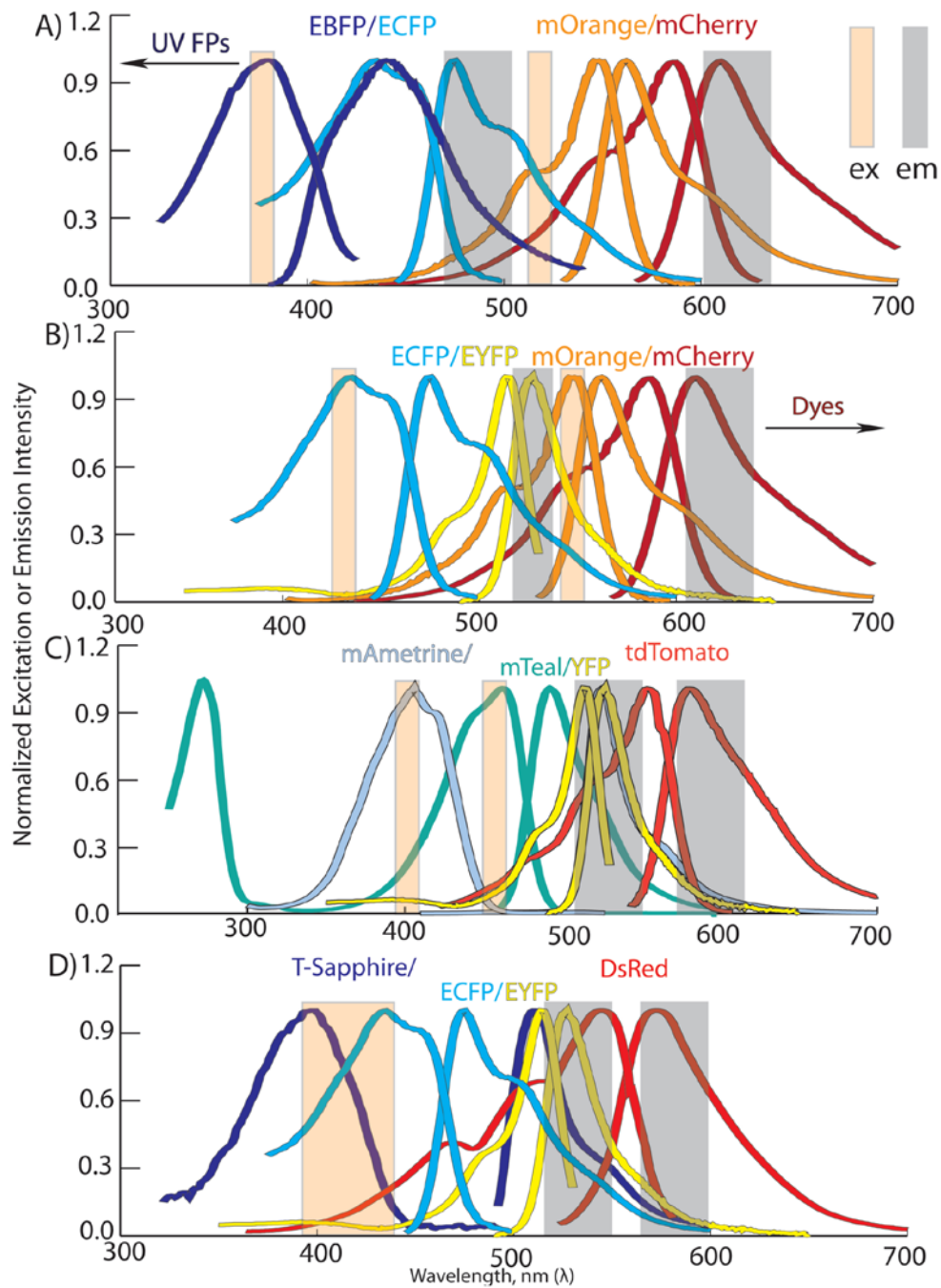
Supplementary information S1 (Figure) | Spectra of fluorophores used in ratiometric FRET multiplex experiments. A) EBFP/ECFP and mOrange/mCherry; B) ECFP/EYFP and mOrange2/mCherry; C) mAmetrine/tdTomato and mTeal/YFP; D) T-Sapphire/DsRed and ECFP/EYFP. The shaded boxes marked “ex” and “em” indicate suggested excitation and emission wavelengths. Spectral data adapted from sources described in McNamara et al. 1
