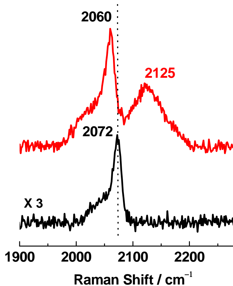
Supplementary Figure 5 | SERS or SHINERS study of CO adsorbed on Pt single-crystal surface. The SERS spectrum of CO on Pt(111) at 0.0 V using bare Au NPs (top), and the SHINERS spectrum of CO on Pt(111) at 0.0 V using Au@SiO 2 NPs (bottom).
