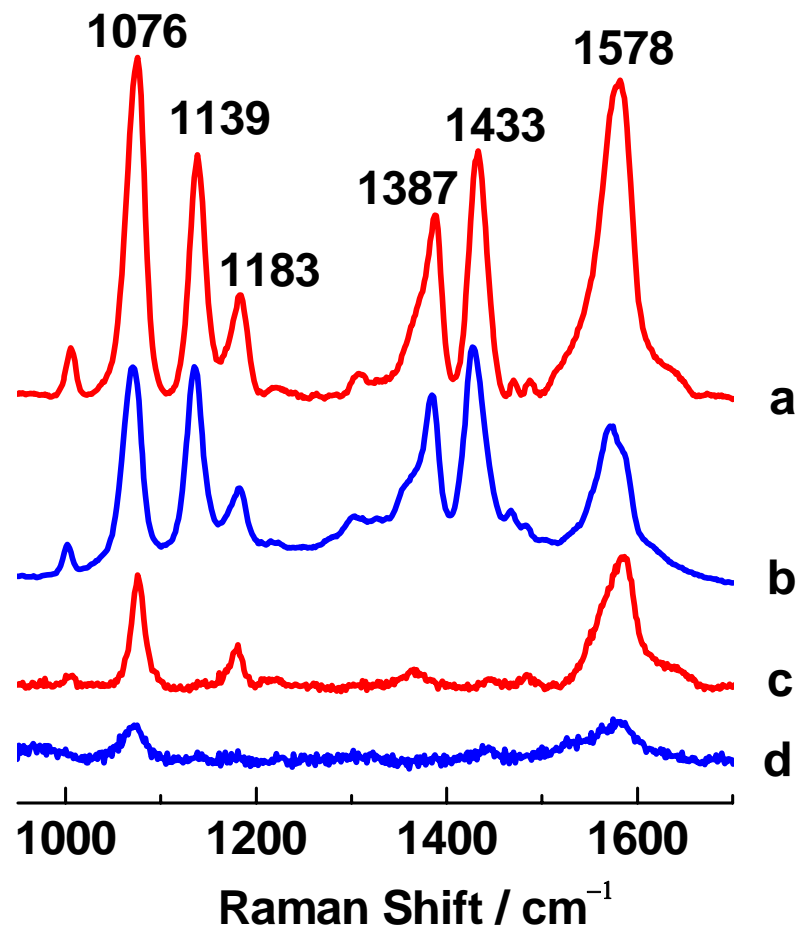
Supplementary Figure 4 | SERS or SHINERS spectra of PATP molecules in different sandwich configurations. (a) Au/PATP/Au NPs, (b) ZnO nanorods/PATP/Au NPs, (c) Au/PATP/Au@SiO 2 NPs, and (d) ZnO nanorods/PATP/Au@SiO 2 NPs.
