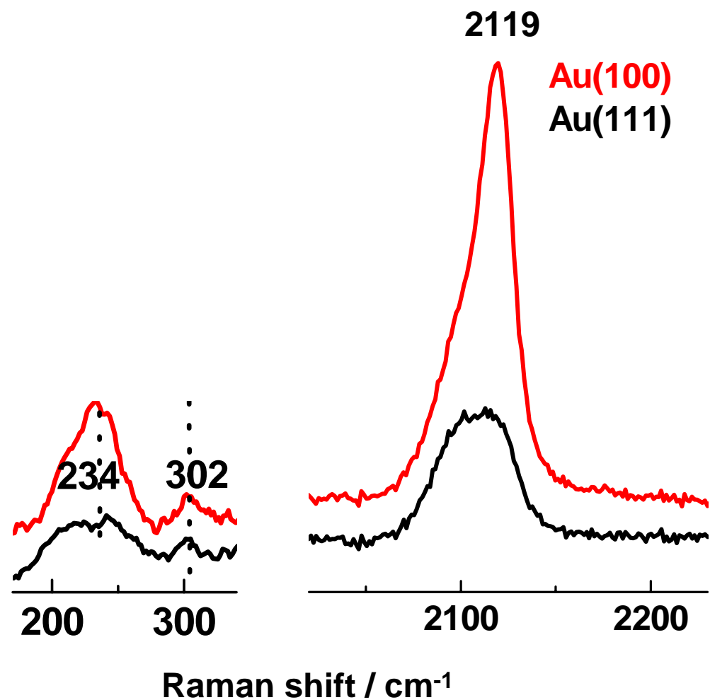
Supplementary Figure 3 | Comparison of the adsorption of SCN - on Au single-crystal surface with different facets. SHINERS spectra of SCN - adsorbed on Au(100) (red curves) and Au(111) (black curves) at 0.0 V.
