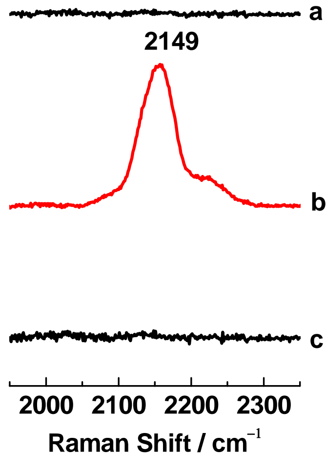
Supplementary Figure 2 | Detection of hydrogen adsorption on Si single-crystal surface. SHINERS spectra obtained from Si(111) treated with (a) sulphuric acid, (b) a 30% HF solution, and (c) an oxygen plasma.
