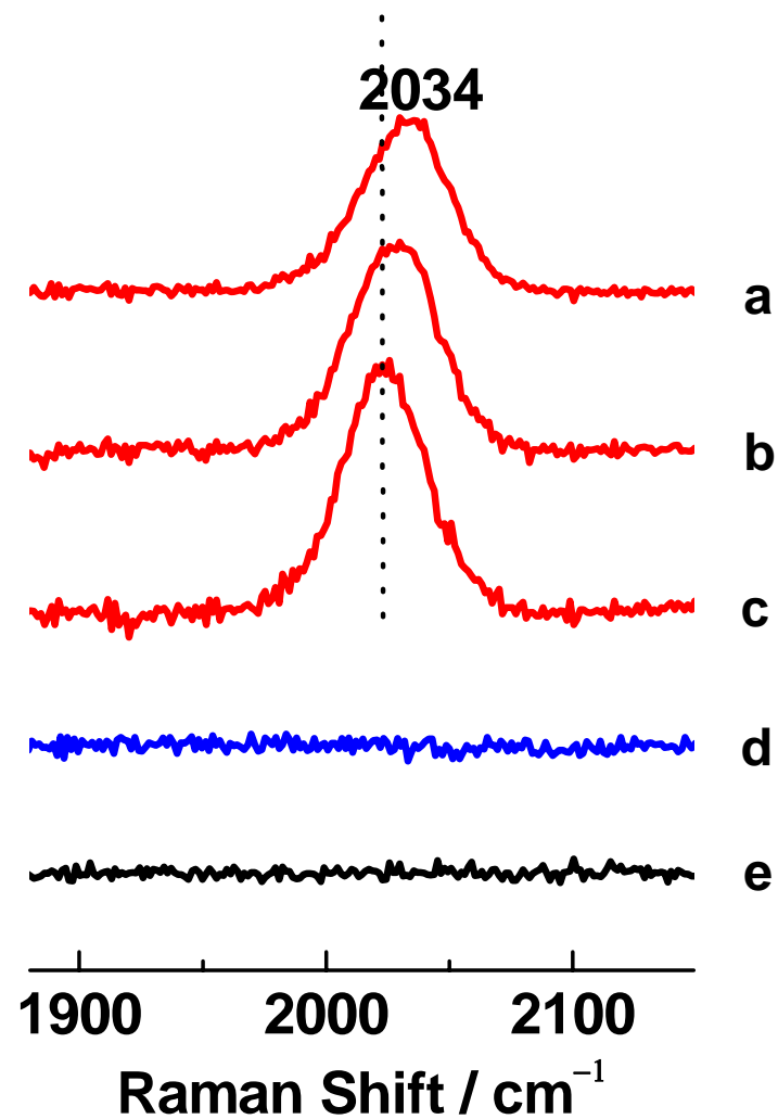
Supplementary Figure 1 | Detection of hydrogen adsorption on Pt single-crystal surface. SHINERS spectra of hydrogen adsorbed on Pt(111) at -1.2 V (a) , at -1.6 V (b) , at -1.9 V (c) , without Au@SiO 2 NPs at -1.9 V (d) , and with the thicker-shell NPs at -1.9 V (e) .
