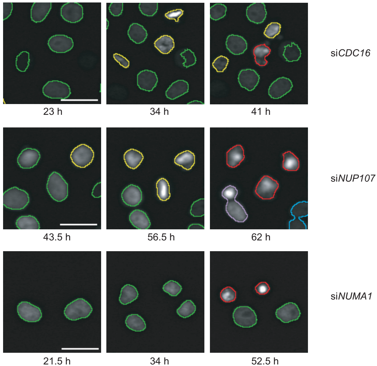
Examples of detected RNAi phenotypes. Phenotypes after knock-down of three additional genes representing different phenotypic classes. CDC16 and NUP107 siRNAs illustrate mitotic (yellow) phenotype followed by apoptosis (red). NUMA1 siRNA illustrates an atypical cell death (red), partially misclassified as mitotic (data not shown). ( Supplementary Movies 5-7 ).
