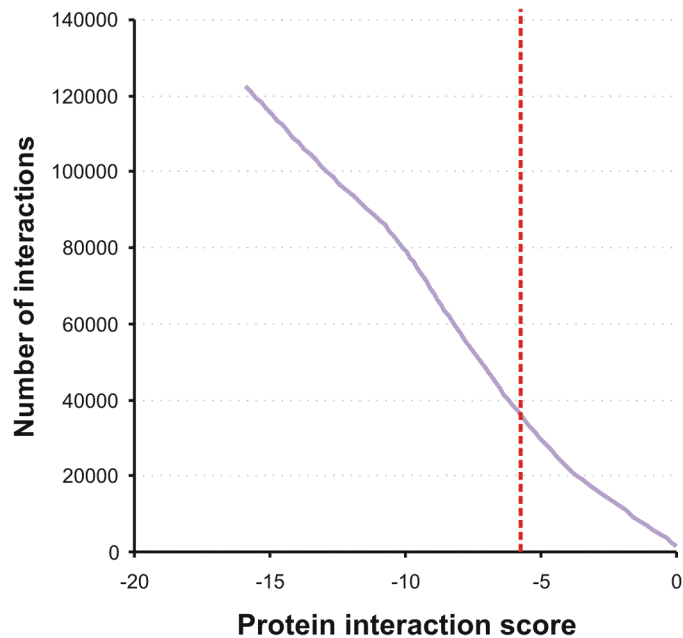
b Number of Interactions as a function of score (not including High Confidence set)
