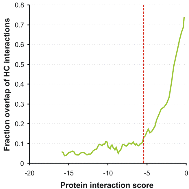
a Overlap of High Confidence interactions as function of score
