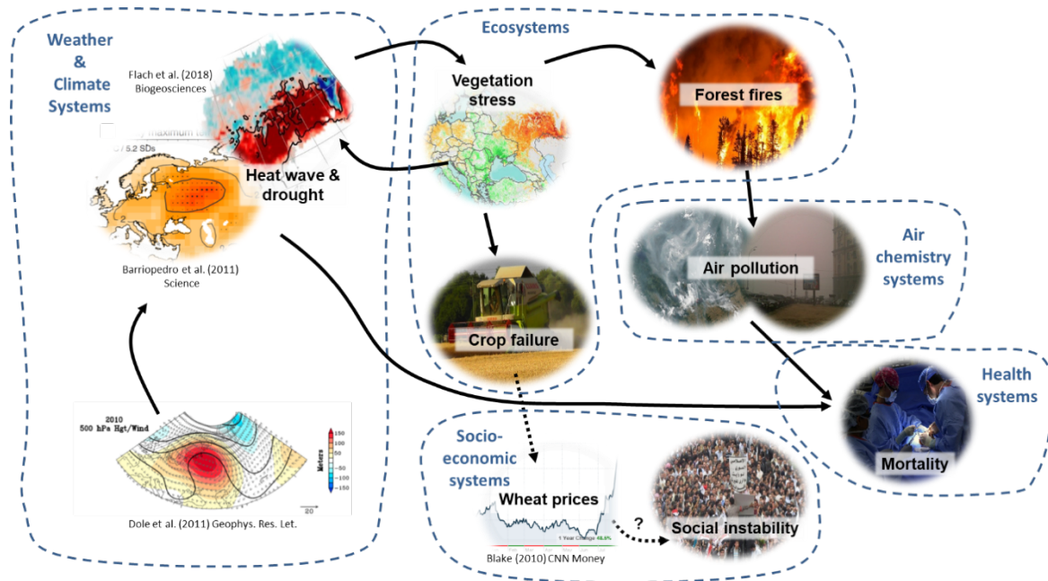
Supplementary Figure S1: Systemic effects of climate extremes exemplified by the Russian heatwave. These effects can transcend sectors and span across country borders, such as the hypothesized social instability with the Arab Spring.
