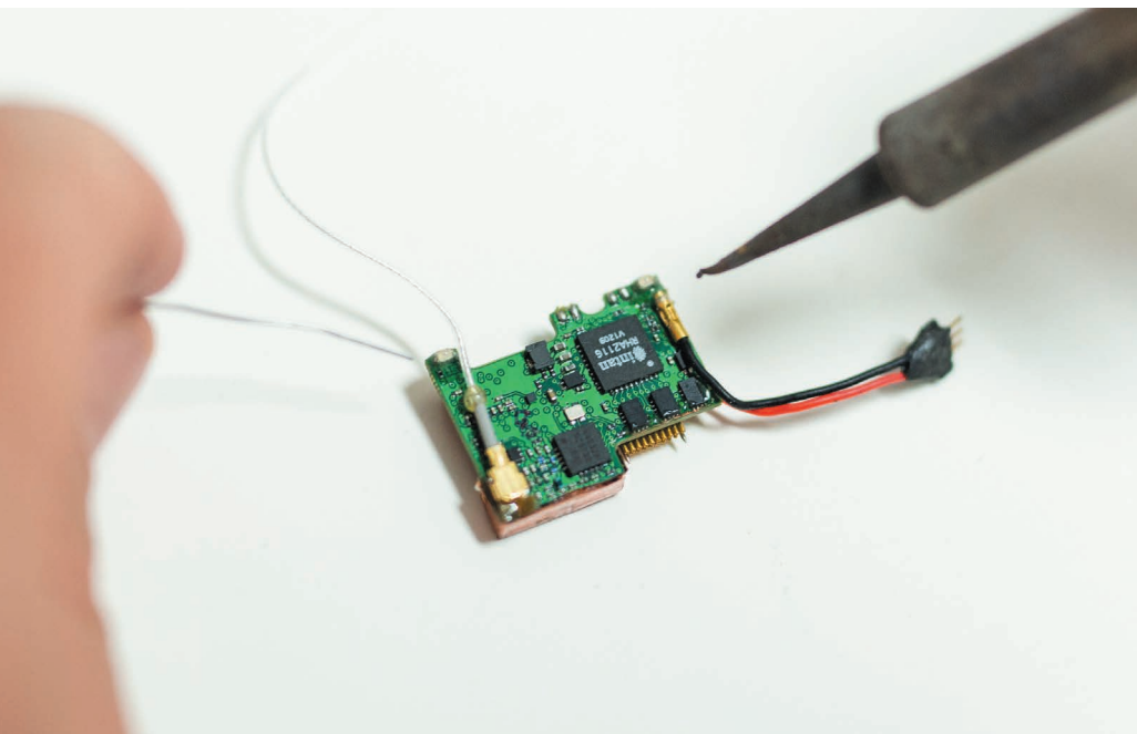
A neural logger designed for wireless recording of neurons in flying bats.
